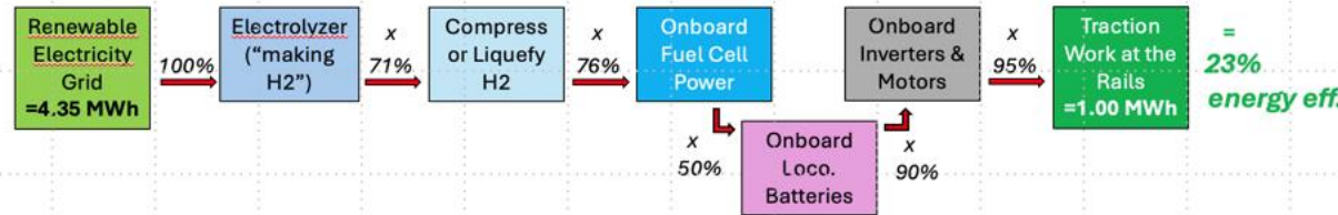
H2 Fuel Cell w/ Batteries Loco.
