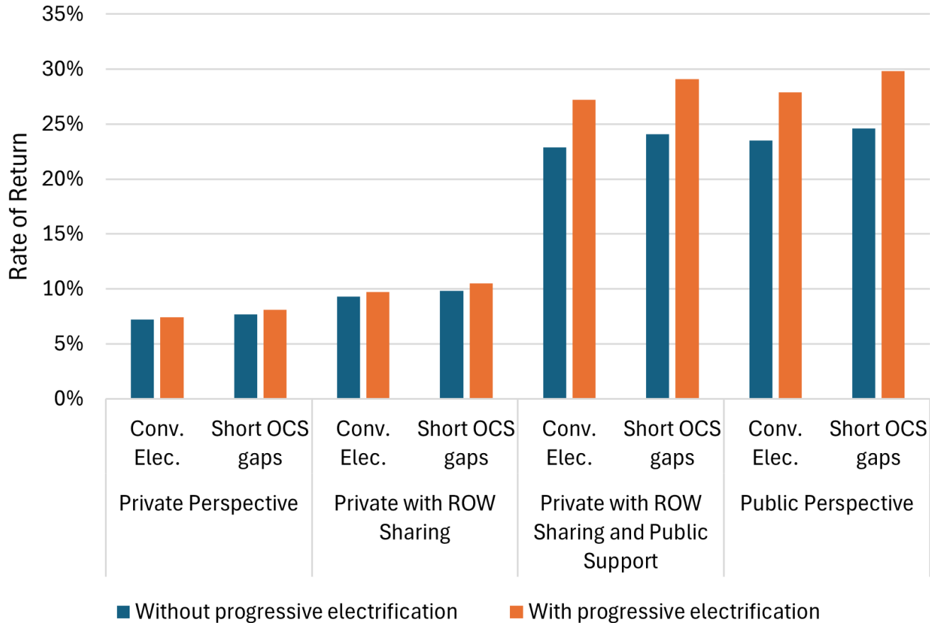
Effect of progressive electrification with dual-mode locomotives
