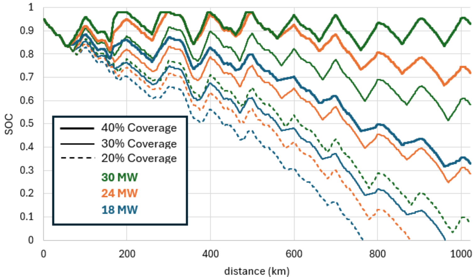
EB Intermodal SOC for different OCS coverage & power configurations
