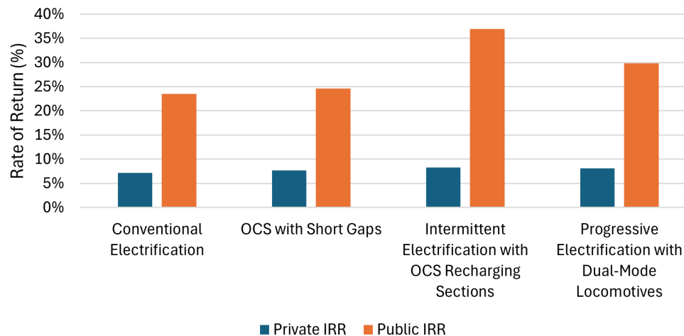
Public & Private Rates of Return for Mainline Electrification Scenarios
