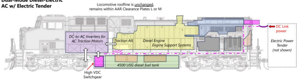
Dual-Mode Diesel-Electric AC w/ Electric Tender
