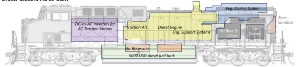
Diesel-Electric AC as-built
