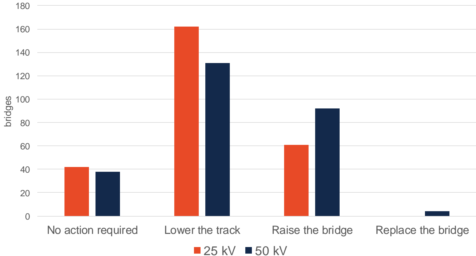
Voltage effect on bridge clearance in the LA basin
